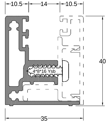
Alt-Yan Kasa Profili BOTTOM-SIDE FRAME PROFILE
