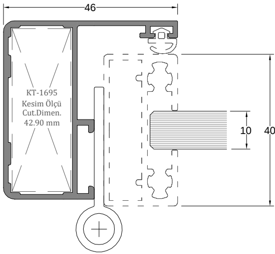
Kasa Profili FRAME PROFILE
